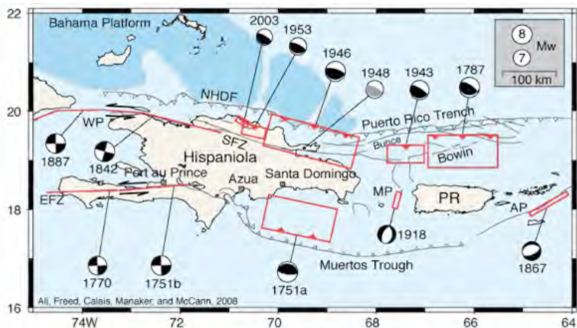
Figure 13. Focal mechanisms and surface projections of estimated rupture planes/geometries for large ( M > 7.0 ) historic and a recent M 6.5 earthquakes in the Gonave microplate boundaries region since 1751. (Acronyms - NHDF: North Hispaniola Deformation Front; NHF: North Hispaniola Fault; WP: Windward Passage; EFZ: Enriquillo Fault Zone; SFZ: Septentrional Fault Zone; MP: Mona Passage; PR: Puerto Rico) (From Ali et al., 2008).
