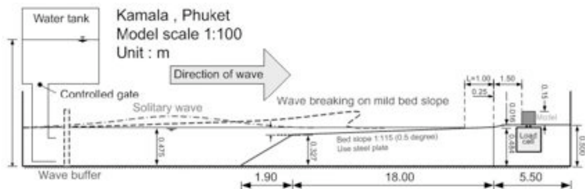
Figure 1 Experimental set-up
