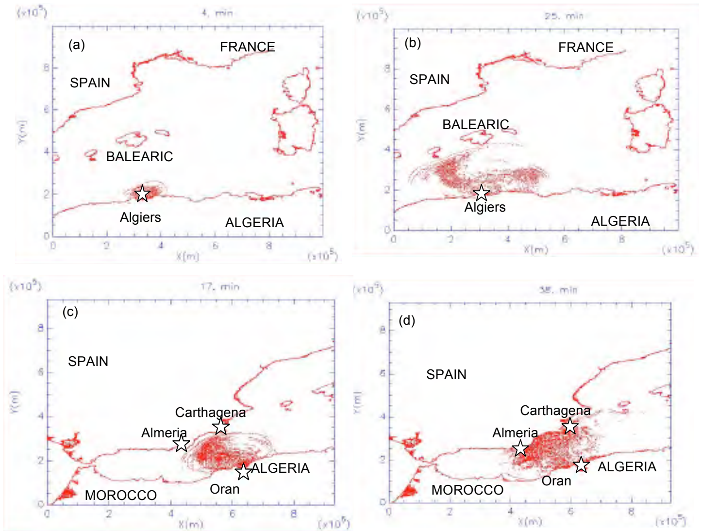
Fig. 5: Tsunami wave propagation for (a & b) Algiers and (c & d) Oran-Alboran study cases. The times are 4 and 25 min for Algiers and 17 and 38 min for Oran. The grid size is 2 min for Algiers and 1 min for Oran-Alboran.
