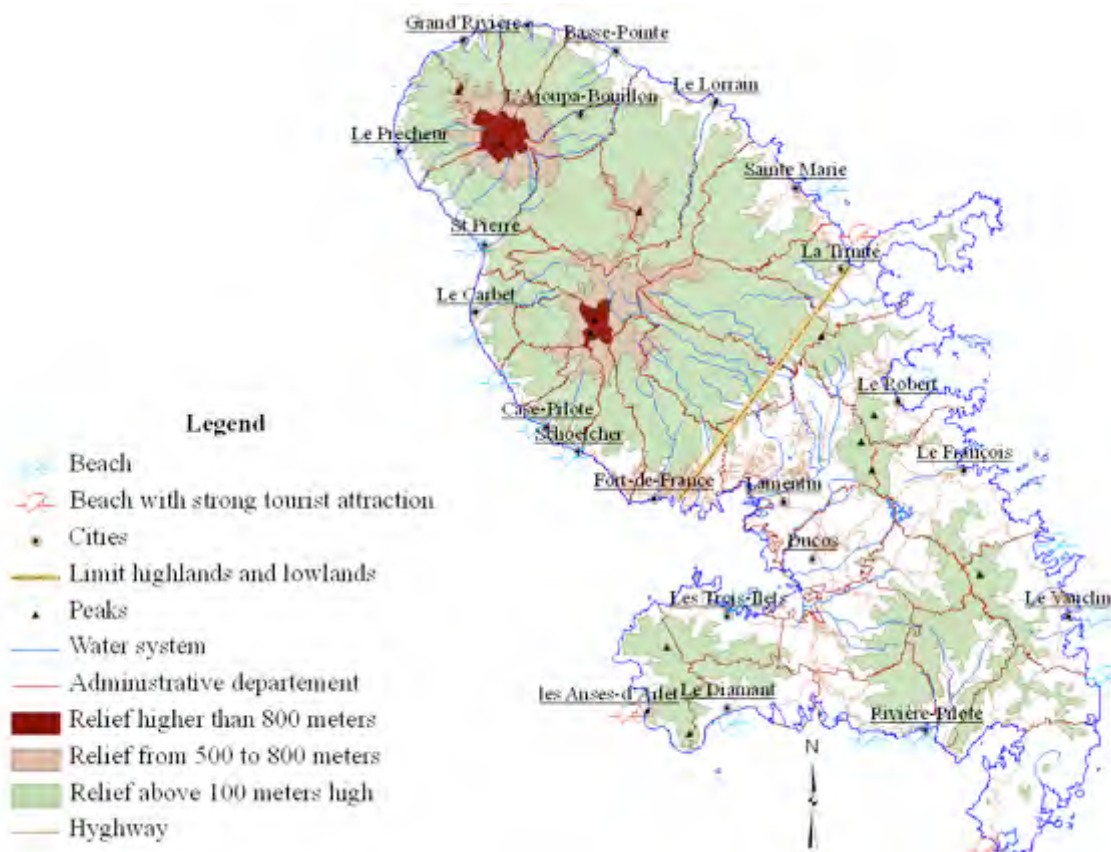
Fig. 2: Geography of Martinique Island. The yellow line indicates the limit between the hilly landscape (northern part) and the plain (southern part).
