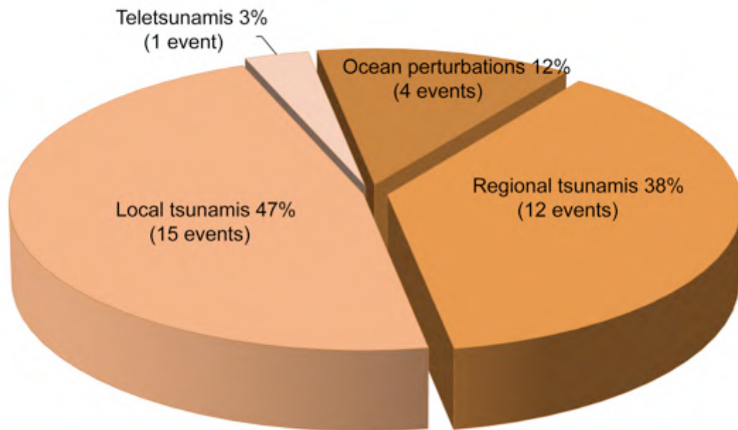
Fig. 5. Classification of tsunamis according to impacted zone.
